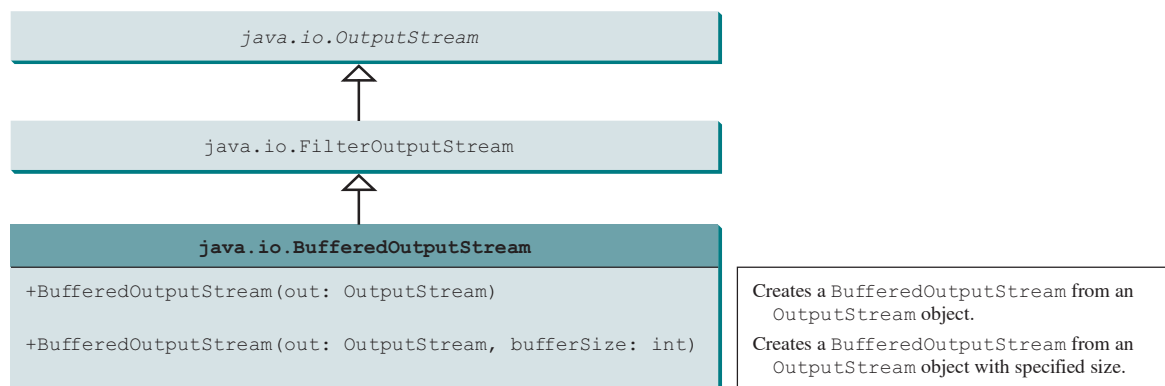
FIGURE 17.14 BufferedOutputStream buffers an output stream.
