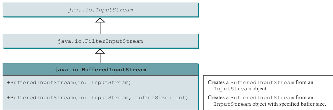
FIGURE 17.13 BufferedInputStream buffers an input stream.
