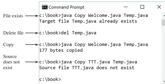
FIGURE 17.15 The program copies a file. Source: Copyright © 1995–2016 Oracle and/or its affiliates. All rights reserved. Used with permission.
