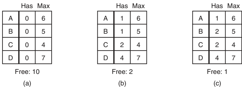
Figure 6-11. Three resource allocation states: (a) Safe. (b) Safe. (c) Unsafe.
