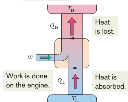
Fig. 20-14 The elements of a refrigerator. The two black arrowheads on the central loop suggest the working substance operating in a cycle, as if on a p - V plot. Energy is transferred as heat Q_L to the working substance from the low-temperature reservoir. Energy is transferred as heat Q_H to the high-temperature reservoir from the working substance. Work W is done on the refrigerator (on the working substance) by something in the environment.
