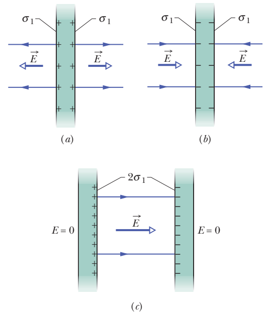
Fig. 23-16 (a) A thin, very large conducting plate with excess positive charge. (b) An identical plate with excess negative charge. (c) The two plates arranged so they are parallel and close.
