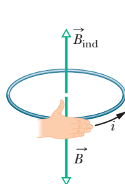
Fig. 30-5 The direction of the current i induced in a loop is such that the current's magnetic field \vec{B}_{\text{ind}} opposes the change in the magnetic field \vec{B} inducing i . The field \vec{B}_{\text{ind}} is always directed opposite an increasing field \vec{B} (a, c) and in the same direction as a decreasing field \vec{B} (b, d). The curled–straight right-hand rule gives the direction of the induced current based on the direction of the induced field.
