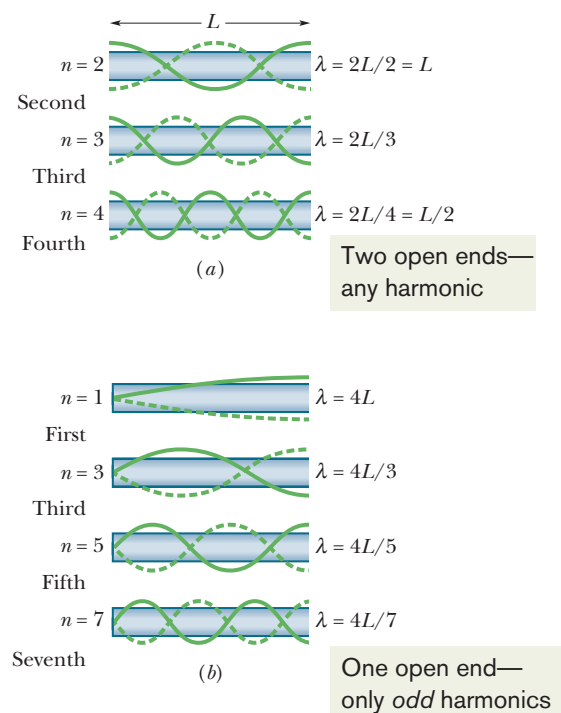
Fig. 17-14 Standing wave patterns for string waves superimposed on pipes to represent standing sound wave patterns in the pipes. (a) With both ends of the pipe open, any harmonic can be set up in the pipe. (b) With only one end open, only odd harmonics can be set up.
