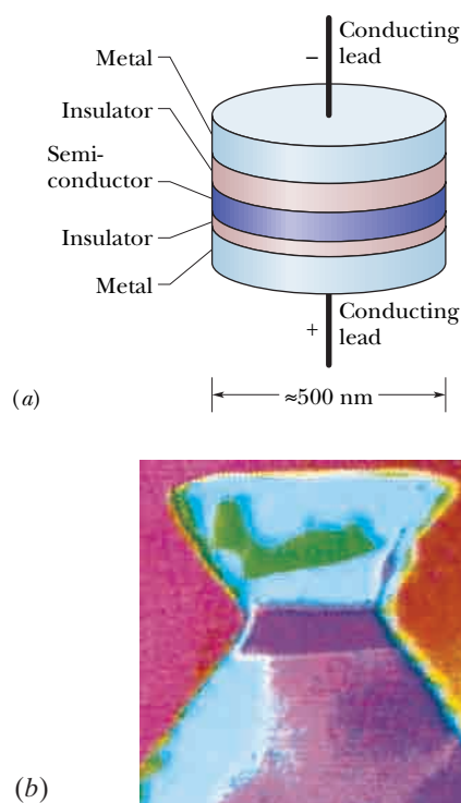
Fig. 39-11 A quantum dot, or “artificial atom.” (a) A central semiconducting layer forms a potential energy well in which electrons are trapped. The lower insulating layer is thin enough to allow electrons to be added to or removed from the central layer by barrier tunneling if an appropriate voltage is applied between the leads. (b) A photograph of an actual quantum dot. The central purple band is the electron confinement region. (From Scientific American, September 1995, page 67. Image reproduced with permission of H. Temkin, Texas Tech University)
