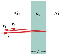
Fig. 35-17 Reflections from a thin film in air.
