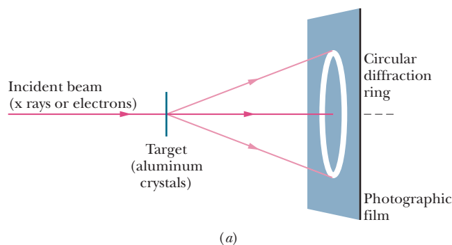
Fig. 38-9 (a) An experimental arrangement used to demonstrate, by diffraction techniques, the wave-like character of the incident beam. Photographs of the diffraction patterns when the incident beam is (b) an x-ray beam (light wave) and (c) an electron beam (matter wave). Note that the two patterns are geometrically identical to each other. (Photo (b) Cameca, Inc. Photo (c) from PSSC film "Matter Waves," courtesy Education Development Center, Newton, Massachusetts)
