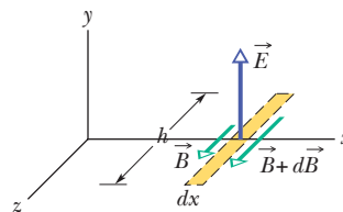
Fig. 33-7 The sinusoidal variation of the electric field through this rectangle, located (but not shown) at point P in Fig. 33-5b, induces magnetic fields along the rectangle. The instant shown is that of Fig. 33-6: \vec{E} is decreasing in magnitude, and the magnitude of the induced magnetic field is greater on the right side of the rectangle than on the left.
