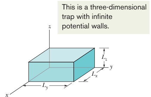
Fig. 39-14 A rectangular box—a three-dimensional version of the infinite potential well of Fig. 39-2—with widths L_x , L_y , and L_z .
