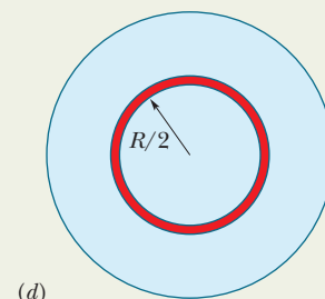
Fig. 26-6 (a) Cross section of a wire of radius R . If the current density is uniform, the current is just the product of the current density and the area. (b) – (e) If the current is nonuniform, we must first find the current through a thin ring and then sum (via integration) the currents in all such rings in the given area.
