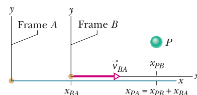
Fig. 4-18 Alex (frame A ) and Barbara (frame B ) watch car P , as both B and P move at different velocities along the common x axis of the two frames. At the instant shown, x_{BA} is the coordinate of B in the A frame. Also, P is at coordinate x_{PB} in the B frame and coordinate x_{PA} = x_{PB} + x_{BA} in the A frame.
