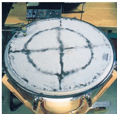
Fig. 16-21 One of many possible standing wave patterns for a kettledrum head, made visible by dark powder sprinkled on the drumhead. As the head is set into oscillation at a single frequency by a mechanical oscillator at the upper left of the photograph, the powder collects at the nodes, which are circles and straight lines in this two-dimensional example. (Courtesy Thomas D. Rossing, Northern Illinois University)
