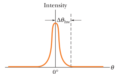
Fig. 36-21 The half-width \Delta\theta_{\text{hw}} of the central line is measured from the center of that line to the adjacent minimum on a plot of I versus \theta like Fig. 36-19a.
