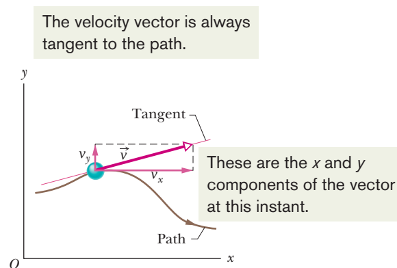
Fig. 4-4 The velocity \vec{v} of a particle, along with the scalar components of \vec{v} .
