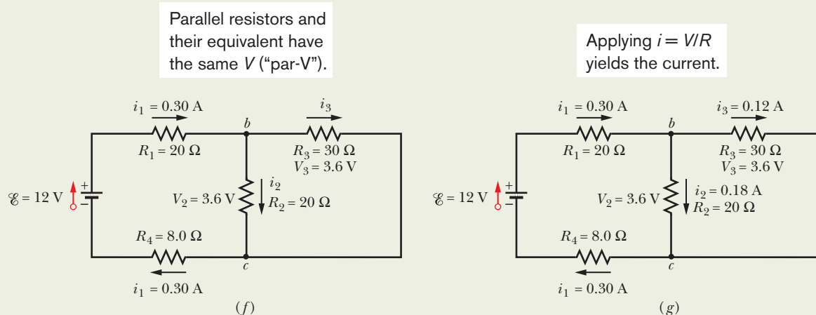
Fig. 27-11 (a) A circuit with an ideal battery. (b) Label the currents. (c) Replacing the parallel resistors with their equivalent. (d)–(g) Working backward to find the currents through the parallel resistors.
