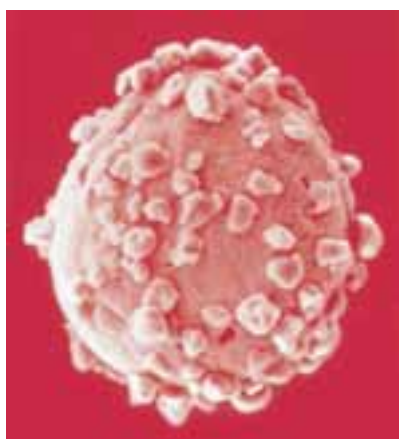
Fig. 21-3 A carrier bead from a photocopying machine; the bead is covered with toner particles that cling to it by electrostatic attraction. The diameter of the bead is about 0.3 mm. (Courtesy Xerox)
