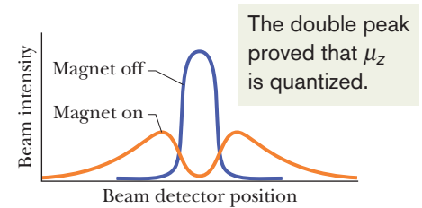
Fig. 40-9 Results of a modern repetition of the Stern–Gerlach experiment. With the electromagnet turned off, there is only a single beam; with the electromagnet turned on, the original beam splits into two subbeams. The two subbeams correspond to parallel and antiparallel alignment of the magnetic moments of cesium atoms with the external magnetic field.
