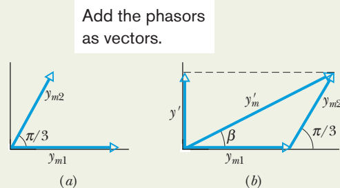
Fig. 16-15 (a) Two phasors of magnitudes y_{m1} and y_{m2} and with phase difference \pi/3 . (b) Vector addition of these phasors at any instant during their rotation gives the magnitude y'_m of the phasor for the resultant wave.
