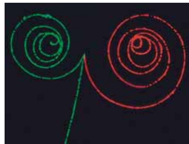
Fig. 38-10 A bubble-chamber image showing where two electrons (paths color coded green) and one positron (red) moved after a gamma ray entered the chamber. (Lawrence Berkeley Laboratory/Science Photo Library/Photo Researchers)
