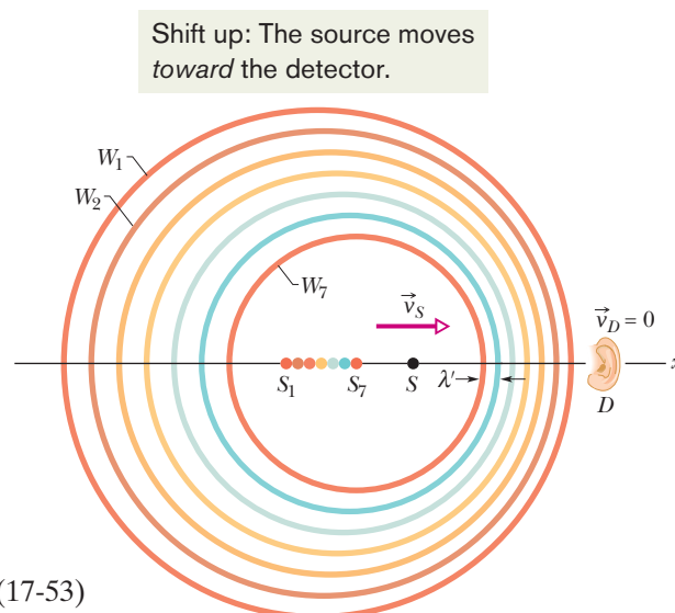
Fig. 17-21 A detector D is stationary, and a source S is moving toward it at speed v_S . Wavefront W_1 was emitted when the source was at S_1 , wavefront W_7 when it was at S_7 . At the moment depicted, the source is at S . The detector senses a higher frequency because the moving source, chasing its own wavefronts, emits a reduced wavelength \lambda' in the direction of its motion.
