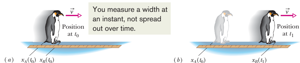
Fig. 37-7 If you want to measure the front-to-back length of a penguin while it is moving, you must mark the positions of its front and back simultaneously (in your reference frame), as in (a), rather than at different times, as in (b).
