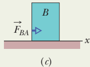
Fig. 5-18 (a) A constant horizontal force \vec{F}_{\text{app}} is applied to block A, which pushes against block B. (b) Two horizontal forces act on block A. (c) Only one horizontal force acts on block B.
