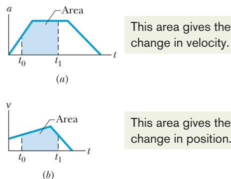
Fig. 2-12 The area between a plotted curve and the horizontal time axis, from time t_0 to time t_1 , is indicated for (a) a graph of acceleration a versus t and (b) a graph of velocity v versus t .
