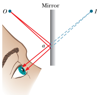
Fig. 34-4 A “pencil” of rays from O enters the eye after reflection at the mirror. Only a small portion of the mirror near a is involved in this reflection. The light appears to originate at point I behind the mirror.
