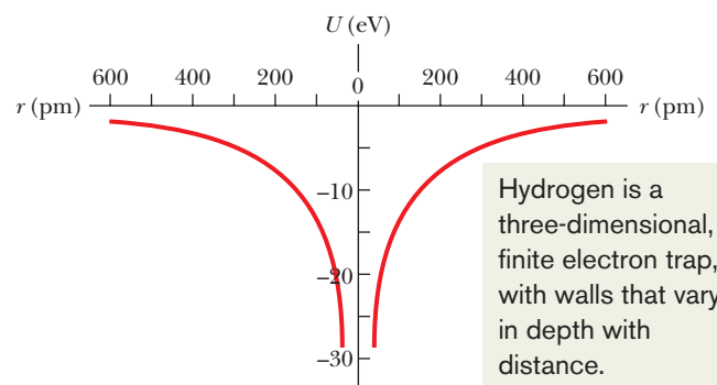
Fig. 39-17 The potential energy U of a hydrogen atom as a function of the separation r between the electron and the central proton. The plot is shown twice (on the left and on the right) to suggest the three-dimensional spherically symmetric trap in which the electron is confined.
