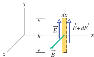
Fig. 33-6 As the electromagnetic wave travels rightward past point P in Fig. 33-5b, the sinusoidal variation of the magnetic field \vec{B} through a rectangle centered at P induces electric fields along the rectangle. At the instant shown, \vec{B} is decreasing in magnitude and the induced electric field is therefore greater in magnitude on the right side of the rectangle than on the left.
