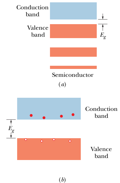
Fig. 41-9 (a) The band-gap pattern for a semiconductor. It resembles that of an insulator (see Fig. 41-4) except that here the energy gap E_g is much smaller; thus electrons, because of their thermal agitation, have some reasonable probability of being able to jump the gap. (b) Thermal agitation has caused a few electrons to jump the gap from the valence band to the conduction band, leaving an equal number of holes in the valence band.
