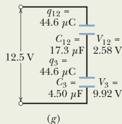
Fig. 25-10 (a) – (d) Three capacitors are reduced to one equivalent capacitor. (e) – (i) Working backwards to get the charges.
