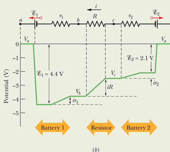
Fig. 27-8 (a) A single-loop circuit containing two real batteries and a resistor. The batteries oppose each other; that is, they tend to send current in opposite directions through the resistor. (b) A graph of the potentials, counterclockwise from point a , with the potential at a arbitrarily taken to be zero. (To better link the circuit with the graph, mentally cut the circuit at a and then unfold the left side of the circuit toward the left and the right side of the circuit toward the right.)
