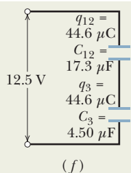
Fig. 25-10 (a) – (d) Three capacitors are reduced to one equivalent capacitor. (e) – (i) Working backwards to get the charges.
