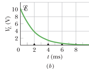
Fig. 30-17 The variation with time of (a) V_R , the potential difference across the resistor in the circuit of Fig. 30-16, and (b) V_L , the potential difference across the inductor in that circuit. The small triangles represent successive intervals of one inductive time constant \tau_L = L/R . The figure is plotted for R = 2000 \Omega , L = 4.0 \text{ H} , and \mathcal{E} = 10 \text{ V} .
