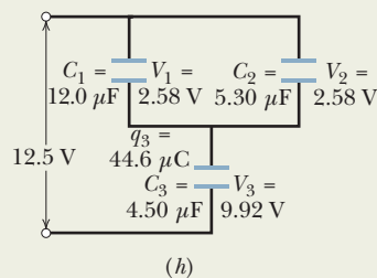
Fig. 25-10 (a) – (d) Three capacitors are reduced to one equivalent capacitor. (e) – (i) Working backwards to get the charges.
