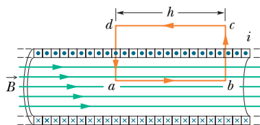
Fig. 29-19 Application of Ampere's law to a section of a long ideal solenoid carrying a current i . The Amperian loop is the rectangle abcda .
