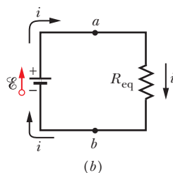
Fig. 27-10 (a) Three resistors connected in parallel across points a and b . (b) An equivalent circuit, with the three resistors replaced with their equivalent resistance R_{eq} .
