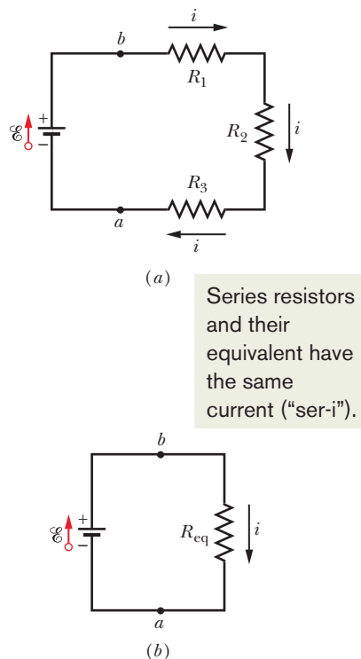
Fig. 27-5 (a) Three resistors are connected in series between points a and b . (b) An equivalent circuit, with the three resistors replaced with their equivalent resistance R_{eq} .
