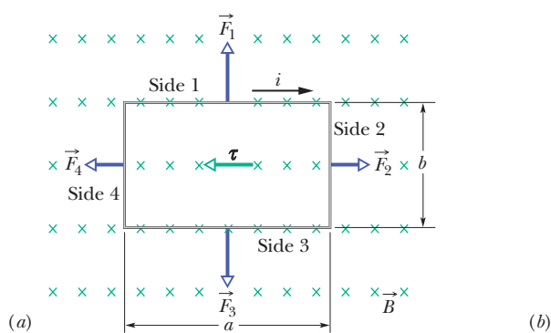
Fig. 28-19 A rectangular loop, of length a and width b and carrying a current i , is located in a uniform magnetic field. A torque \tau acts to align the normal vector \vec{n} with the direction of the field. (a) The loop as seen by looking in the direction of the magnetic field. (b) A perspective of the loop showing how the right-hand rule gives the direction of \vec{n} , which is perpendicular to the plane of the loop. (c) A side view of the loop, from side 2. The loop rotates as indicated.
