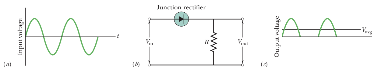
Fig. 41-14 A p - n junction connected as a junction rectifier. The action of the circuit in (b) is to pass the positive half of the input wave form in (a) but to suppress the negative half. The average potential of the input wave form is zero; that of the output wave form in (c) has a positive value V_{\text{avg}} .
