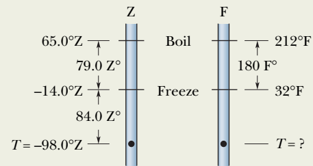
Fig. 18-8 An unknown temperature scale compared with the Fahrenheit temperature scale.
