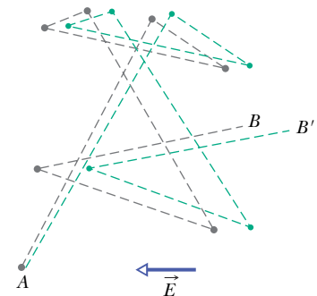
Fig. 26-12 The gray lines show an electron moving from A to B , making six collisions en route. The green lines show what the electron's path might be in the presence of an applied electric field \vec{E} . Note the steady drift in the direction of -\vec{E} . (Actually, the green lines should be slightly curved, to represent the parabolic paths followed by the electrons between collisions, under the influence of an electric field.)
