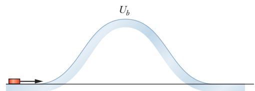
Fig. 38-13 A puck slides over frictionless ice toward a hill. The puck's gravitational potential at the top of the hill will be U_b .
