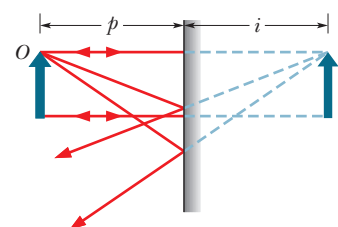
Fig. 34-5 An extended object O and its virtual image I in a plane mirror.
