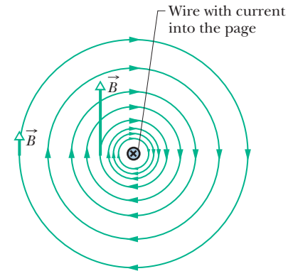
Fig. 29-2 The magnetic field lines produced by a current in a long straight wire form concentric circles around the wire. Here the current is into the page, as indicated by the \times .
