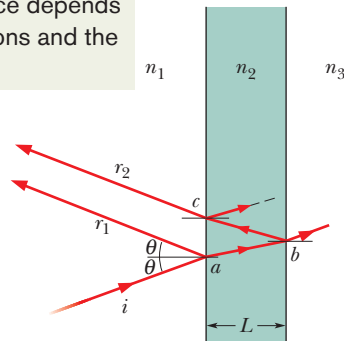
Fig. 35-15 Light waves, represented with ray i , are incident on a thin film of thickness L and index of refraction n_2 . Rays r_1 and r_2 represent light waves that have been reflected by the front and back surfaces of the film, respectively. (All three rays are actually nearly perpendicular to the film.) The interference of the waves of r_1 and r_2 with each other depends on their phase difference. The index of refraction n_1 of the medium at the left can differ from the index of refraction n_3 of the medium at the right, but for now we assume that both media are air, with n_1 = n_3 = 1.0 , which is less than n_2 .
