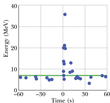
Fig. 42-12 A burst of neutrinos from the supernova SN 1987A, which occurred at (relative) time 0, stands out from the usual background of neutrinos. (For neutrinos, 10 is a “burst.”) The particles were detected by an elaborate detector housed deep in a mine in Japan. The supernova was visible only in the Southern Hemisphere; so the neutrinos had to penetrate Earth (a trifling barrier for them) to reach the detector.
