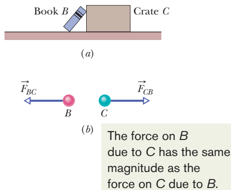
Fig. 5-10 (a) Book B leans against crate C . (b) Forces \vec{F}_{BC} (the force on the book from the crate) and \vec{F}_{CB} (the force on the crate from the book) have the same magnitude and are opposite in direction.
