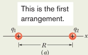
Fig. 21-8 (a) Two charged particles of charges q_1 and q_2 are fixed in place on an x axis. (b) The free-body diagram for particle 1, showing the electrostatic force on it from particle 2. (c) Particle 3 included. (d) Free-body diagram for particle 1. (e) Particle 4 included. (f) Free-body diagram for particle 1.
