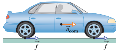
Fig. 8-16 A vehicle accelerates to the right using four-wheel drive. The road exerts four frictional forces (two of them shown) on the bottom surfaces of the tires. Taken together, these four forces make up the net external force \vec{F} acting on the car.
