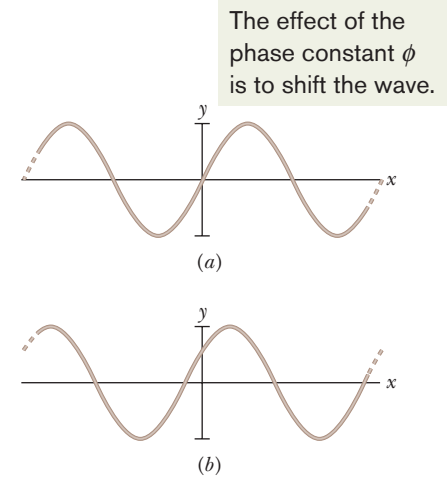
Fig. 16-6 A sinusoidal traveling wave at t = 0 with a phase constant \phi of (a) 0 and (b) \pi/5 rad.
