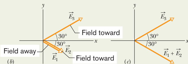
Fig. 22-7 (a) Three particles with charges q_1 , q_2 , and q_3 are at the same distance d from the origin. (b) The electric field vectors \vec{E}_1 , \vec{E}_2 , and \vec{E}_3 at the origin due to the three particles. (c) The electric field vector \vec{E}_3 and the vector sum \vec{E}_1 + \vec{E}_2 at the origin.
