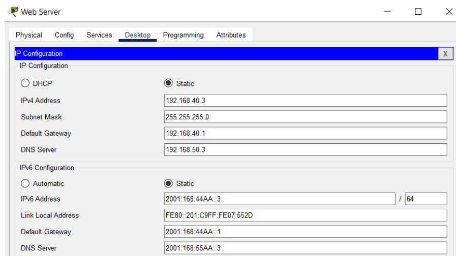
Figure 3: Web server configuration.
