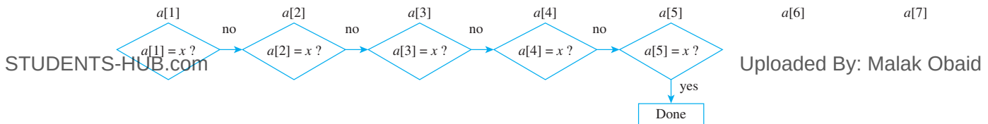
Figure 11.3.1 Sequential Search of a[1], a[2], \dots, a[7] for x where x = a[5]
