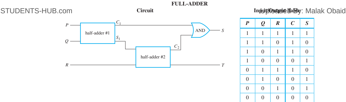
Figure 2.5.2 Circuit to Add P + Q + R , Where P , Q , and R Are Binary Digits
