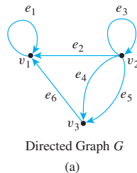
Figure 10.3.1 A Directed Graph and Its Adjacency Matrix
