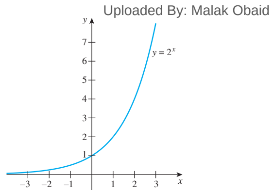
Figure 11.4.1 The Exponential Function with Base 2
