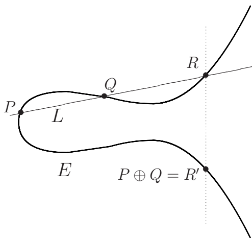
Figure 5.2: The addition law on an elliptic curve
