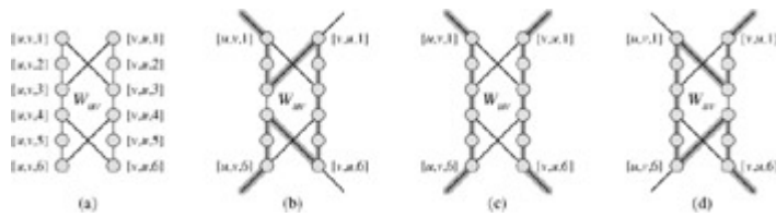
Figure 34.16: The widget used in reducing the vertex-cover problem to the hamiltonian-cycle problem. An edge (u, v) of graph G corresponds to widget W_{uv} in the graph G' created in the reduction. (a) The widget, with individual vertices labeled. (b)-(d) The shaded paths are the only possible ones through the widget that include all vertices, assuming that the only connections from the widget to the remainder of G' are through vertices [u, v, 1] , [u, v, 6] , [v, u, 1] , and [v, u, 6] .
