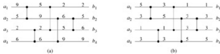
Figure 27.5: (a) The sorting network from Figure 27.2 with input sequence \square 9, 5, 2, 6 \square . (b)
