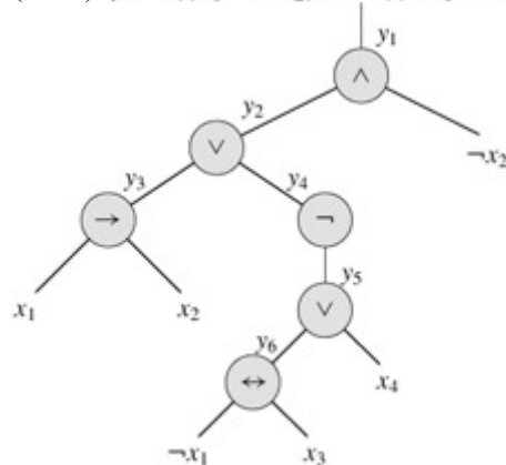
Figure 34.11: The tree corresponding to the formula \phi = ((x_1 \rightarrow x_2) \sqcup \neg((\neg x_1 \leftrightarrow x_3) \sqcup x_4)) \sqcup \neg x_2 .
