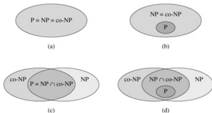
Figure 34.3: Four possibilities for relationships among complexity classes. In each diagram, one region enclosing another indicates a proper-subset relation. (a) \text{P} = \text{NP} = \text{co-NP} . Most researchers regard this possibility as the most unlikely. (b) If NP is closed under complement, then \text{NP} = \text{co-NP} , but it need not be the case that \text{P} = \text{NP} . (c) \text{P} = \text{NP} \cap \text{co-NP} , but NP is not closed under complement. (d) \text{NP} \neq \text{co-NP} and \text{P} \neq \text{NP} \cap \text{co-NP} . Most researchers regard this possibility as the most likely.
