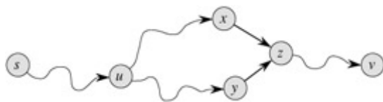
Figure 24.9: Showing that a path in G_\pi from source s to vertex v is unique. If there are two paths p_1 (s \rightsquigarrow u \rightsquigarrow x \rightarrow z \rightsquigarrow v) and p_2 (s \rightsquigarrow u \rightsquigarrow y \rightarrow z \rightsquigarrow v) , where x \neq y , then \pi[z] = x and \pi[z] = y , a contradiction.
