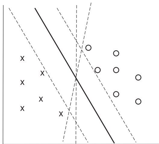
Figure 11.12 Example of a Support Vector Machine classifier.
