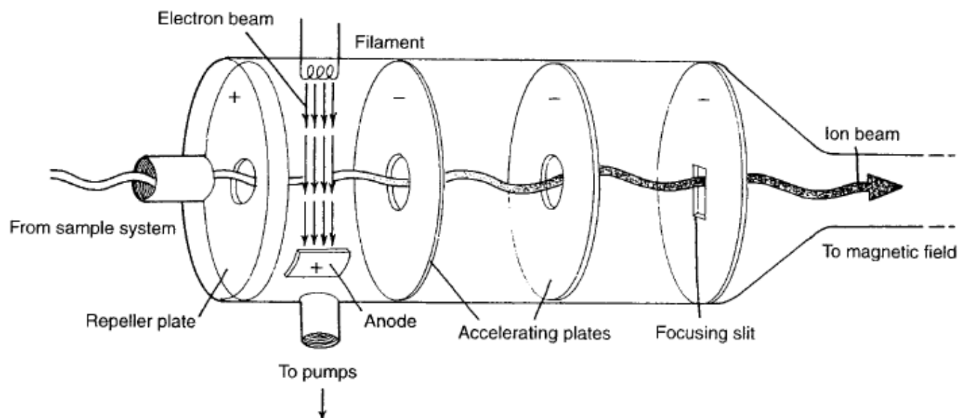
Figure 05.02: A typical ionization chamber and the nearby accelerating plates.
