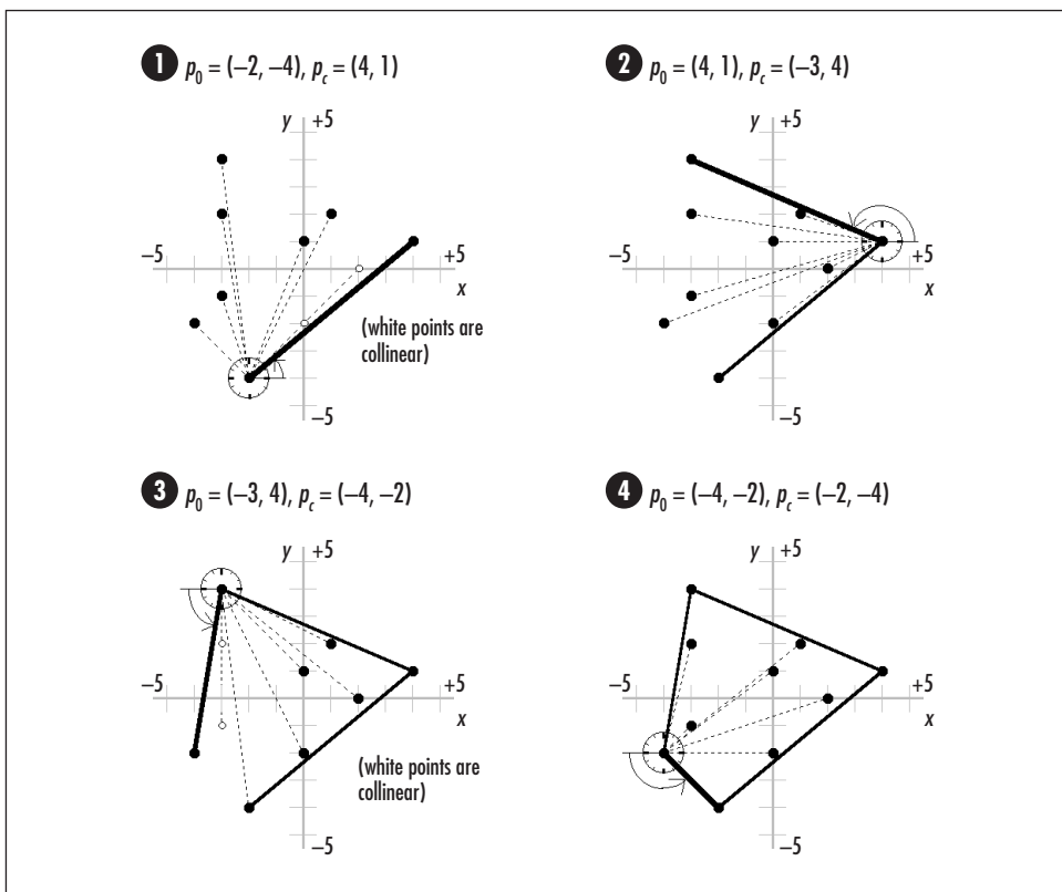
Figure 17-4. Computing the convex hull for a set of 10 points
