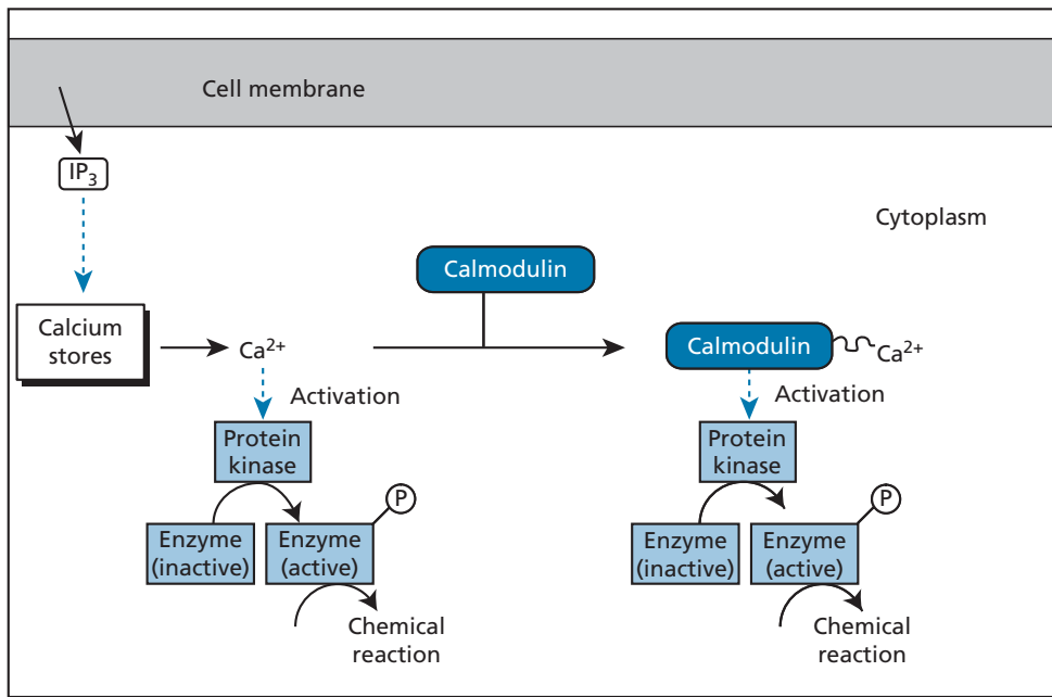
FIGURE 5.12 Signal transduction initiated by inositol triphosphate (IP 3 ). (P = phosphate)
