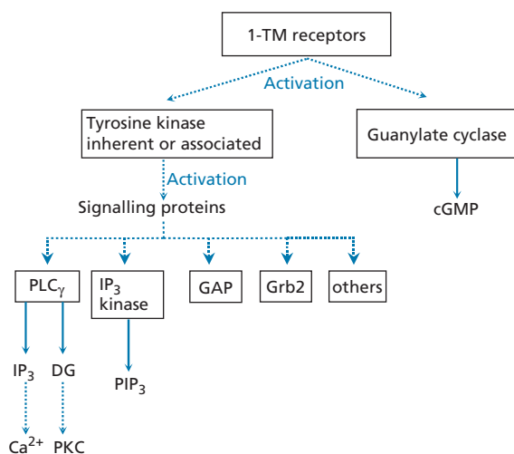
FIGURE 5.15 Signalling pathways from 1-TM receptors.
