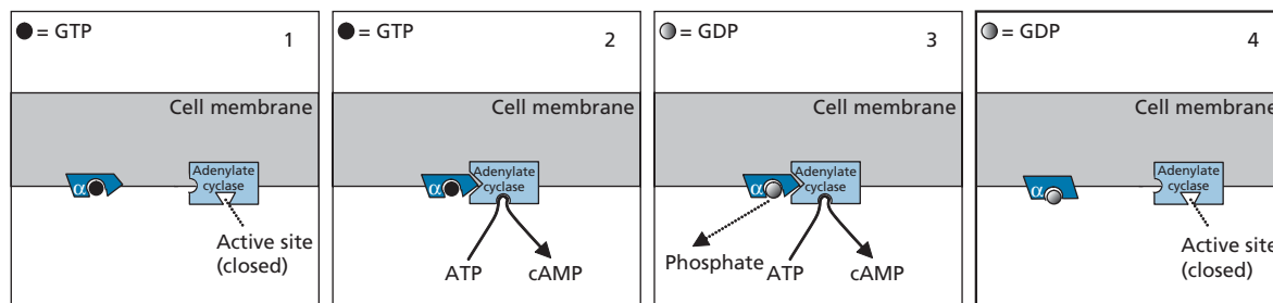
FIGURE 5.3 Interaction of \alpha_s -subunit with adenylylate cyclase and activation of the enzyme.
