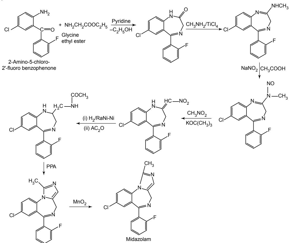
8-Chloro-6-(2-fluorophenyl)-2-methyl-imidazo benzodiazepine
