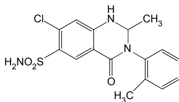
7-Chloro-1,2,3,4-tetrahydro-2-methyl-3-(2-methylphenyl)-4-oxo-6-quinazoline sulphonamide
