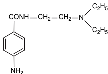
Procainamide
