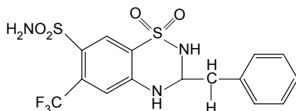
3-Benzyl-3,4-dihydro-6(trifluoromethyl)-2H-1,2,4-benzothiazine-7-sulphonamide-1,1-dioxide
