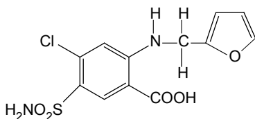
Furosemide
