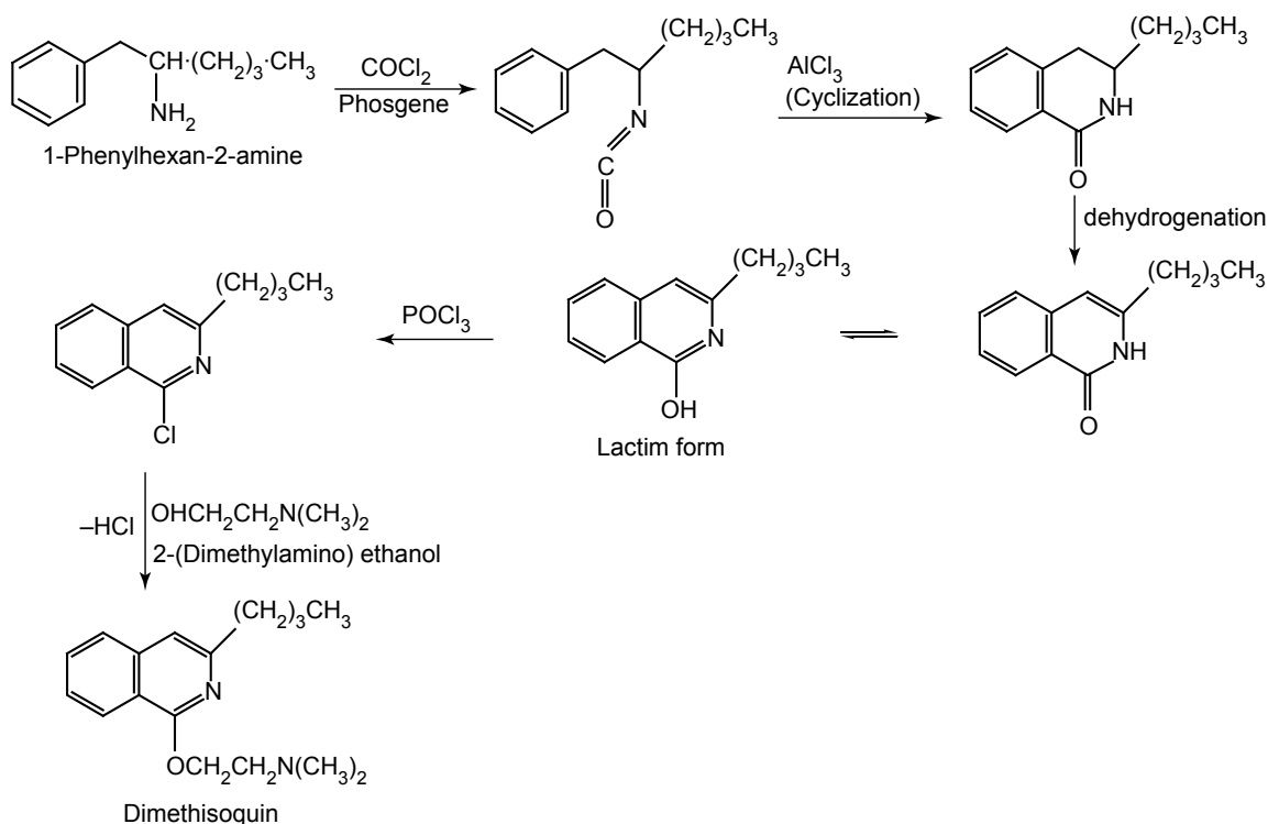
3-Butyl-1-(2-(dimethylamino)ethoxy)isoquinoline
