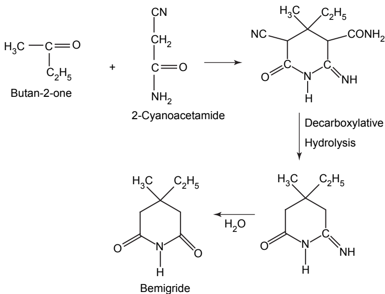
4-Ethyl-4-methylpiperidine-2,6-dione
