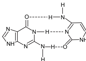
Guanine–cytosine
