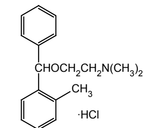
Orphenadrine
