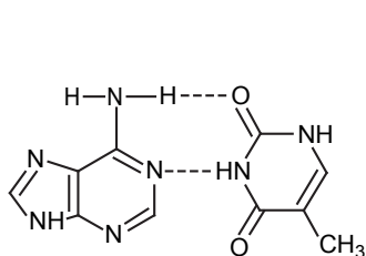
Adenine–thymine
