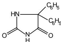
5, 5-Diphenylimidazolidine-2, 4-dione
