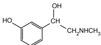
f. Phenylephrine
