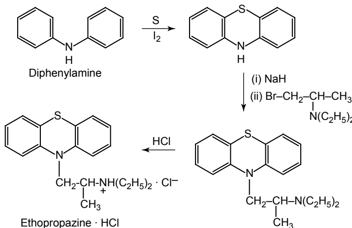
10-[2-(Diethylamino)propyl]phenothiazine hydrochloride
