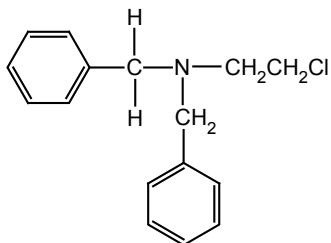
N-(2-Chloro ethyl)-N-Dibenzylamine
