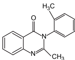
Methaqualone
