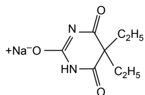
Sodium-5,5'-diethylbarbiturate
