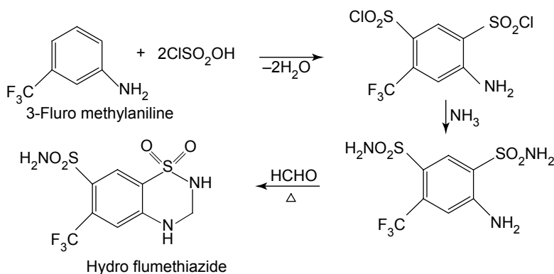
3,4-Dihydro-6(trifluoromethyl)-2H-1,2,4-benzothiazine-7-sulphonamide-1,1-dioxide
