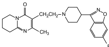
3-[2-[4-(6-Fluoro-1,2-benzisoxazol-3-yl)-1-piperidinyl]ethyl]-6,7,8,9-tetrahydro-2-methyl-4H-pyrido(1,2-a)pyrimidin-4-one
