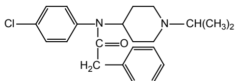
N-(4-Chlorophenyl)-N-(1-isopropylpiperidin-4-yl)-2-phenylacetamide
