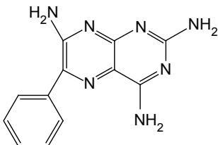
Triamterene
