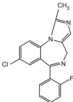
8-Chloro-6-(2-fluorophenyl)-2-methyl-imidazo benzodiazepine
