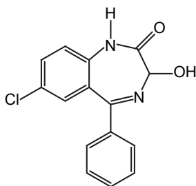
7-Chloro-3-hydroxy-5-phenyl-1,4-benzodiazepin-2-one
