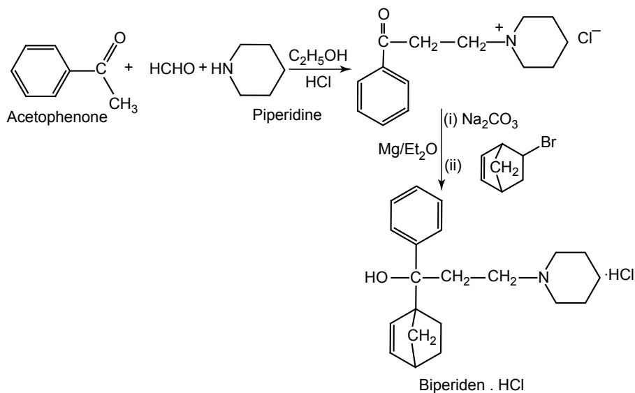
1-(Bicyclo hept-2-en-1-yl)-1-phenyl-3-(piperidin-1-yl)propan-1-ol
