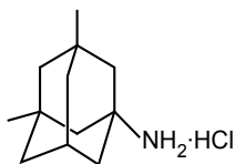
1-Amino-3, 5-dimethyl-adamantane
