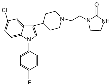
1-(2-(4-(5-Chloro-1-(4-fluorophenyl)-1H-indol-3-yl)piperidin-1-yl)ethyl)imidazolidin-2-one
