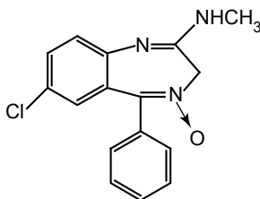
7-Chloro-5-phenyl-2-methylamino-1,4-benzodiazepine-4-oxide
