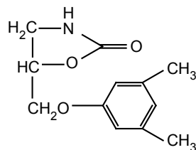
Metaxalone
