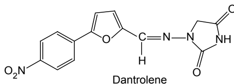
Dantrolene
