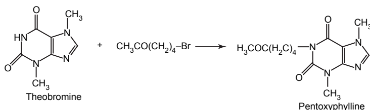
3,7-Dimethyl-1-(5-oxohexyl)-1H-purine-2,6(3H,7H)-dione
