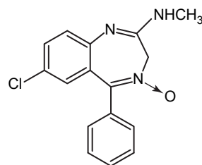
Chlordiazepoxide
