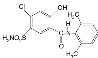
Xipamide (Salicylanilide)
