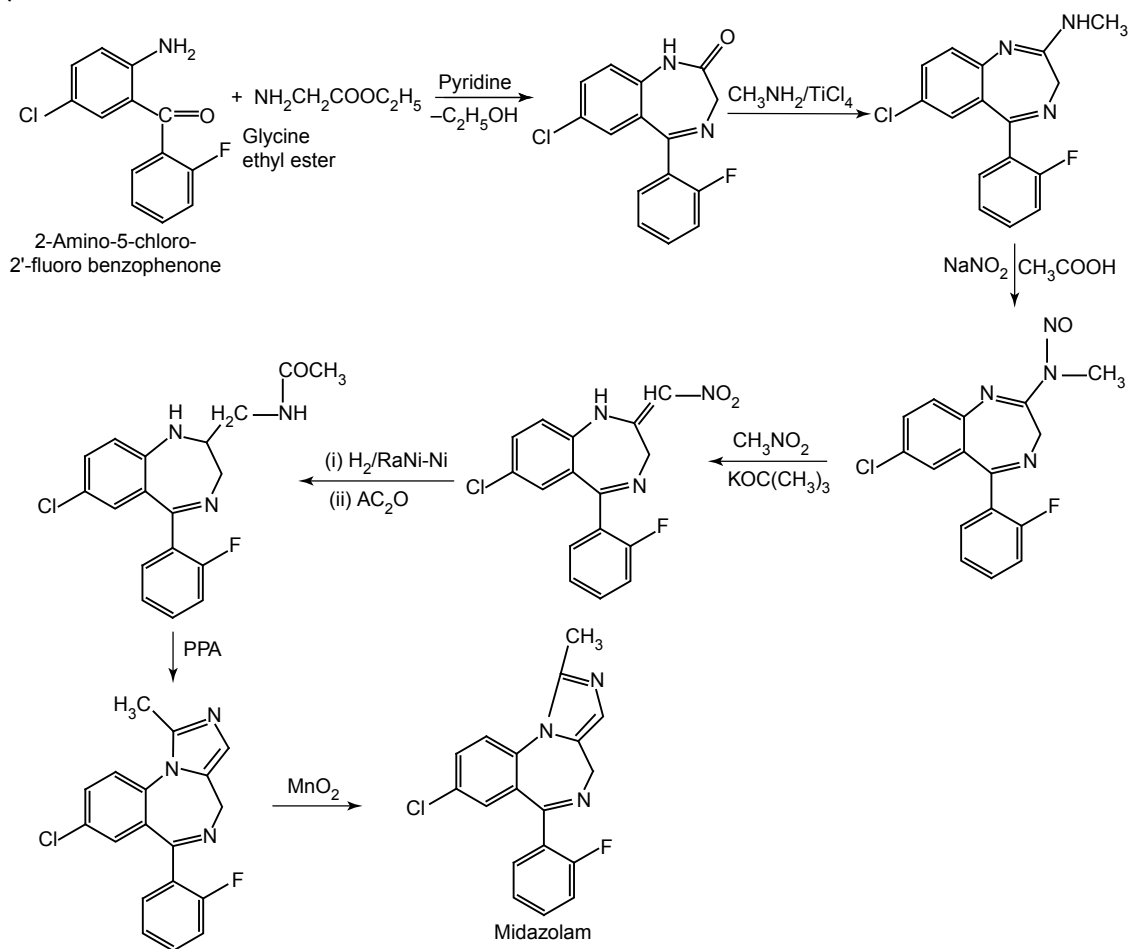
8-Chloro-6-(2-fluorophenyl)-2-methyl-imidazo benzodiazepine
