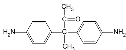
Amphenone B
