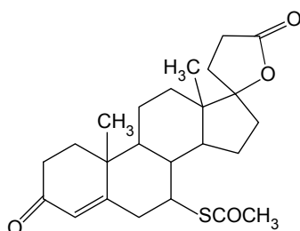
Spironolactone
