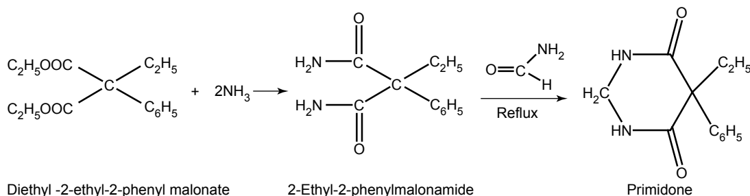
5-Ethyl-2-hydro-5-phenyl-4,6-pyrimidine dione
