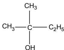
Amylene hydrate
