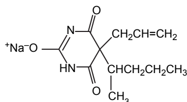
Sodium-5-allyl-5-(1-methylbutyl) barbiturate
