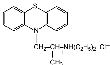
10-[2-(Diethylamino)propyl]phenothiazine hydrochloride
