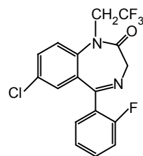
Fletazepam
