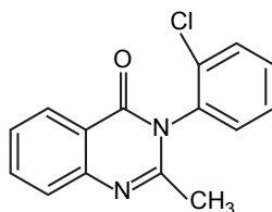
Mecloqualone
