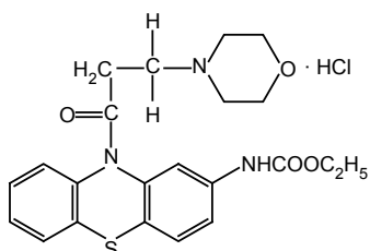
Ethyl-10-(3-morpholinopropanoyl)-phenothiazin-2-yl-carbamate hydrochloride
