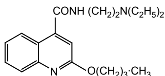
2-Butoxy-N-(2-(diethylamino)ethyl)-4-quinoline carboxamide
