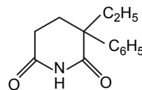
Glutethimide
