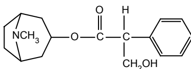
8-Methyl-8-aza-bicyclo[3.2.1]octan-3-yl 3-hydroxy-2-phenylpropanoate
