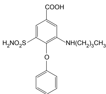
3-Butylamino-4-phenoxy-5-sulphamoylbenzoic acid
