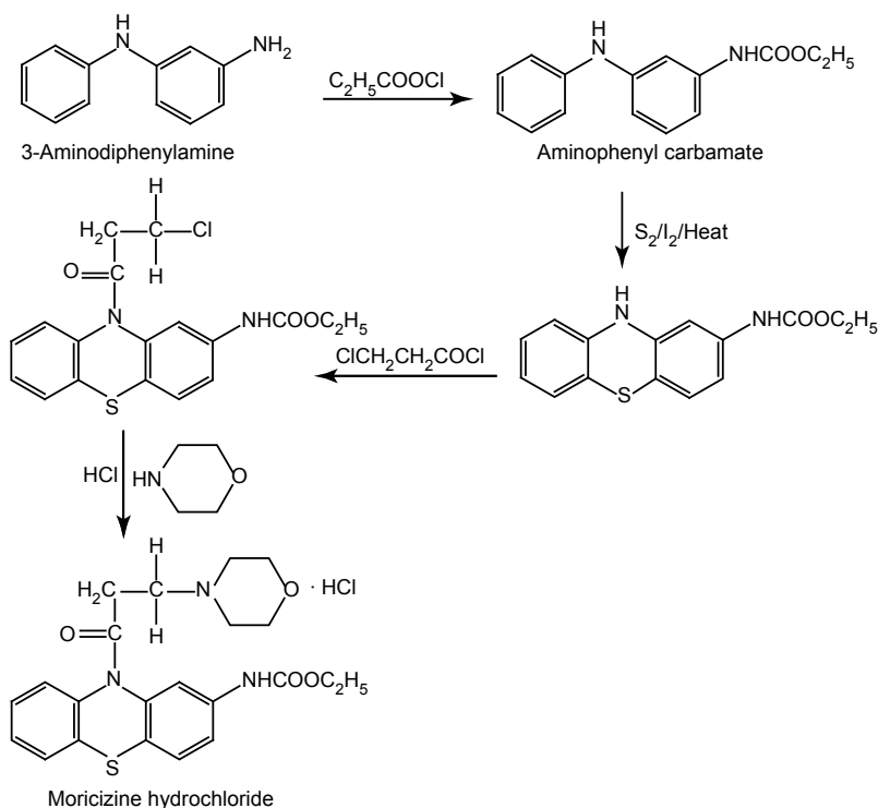
Ethyl-10-(3-morpholinopropanoyl)-phenothiazin-2-yl-carbamate hydrochloride
