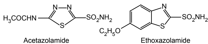
Acetazolamide
