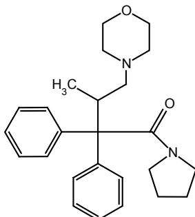
3-Methyl-4-morpholino-2,2-diphenyl-1-(pyrrolidin-1-yl)butan-1-one
