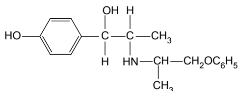
4-(1-Hydroxy-2-(1-phenoxypropyl-amino)propyl) phenol
