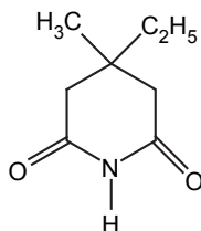
4-Ethyl-4-methylpiperidine-2,6-dione
