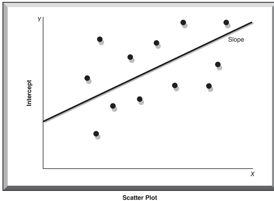
Figure A1.3 Scatter Plot of Y versus X
