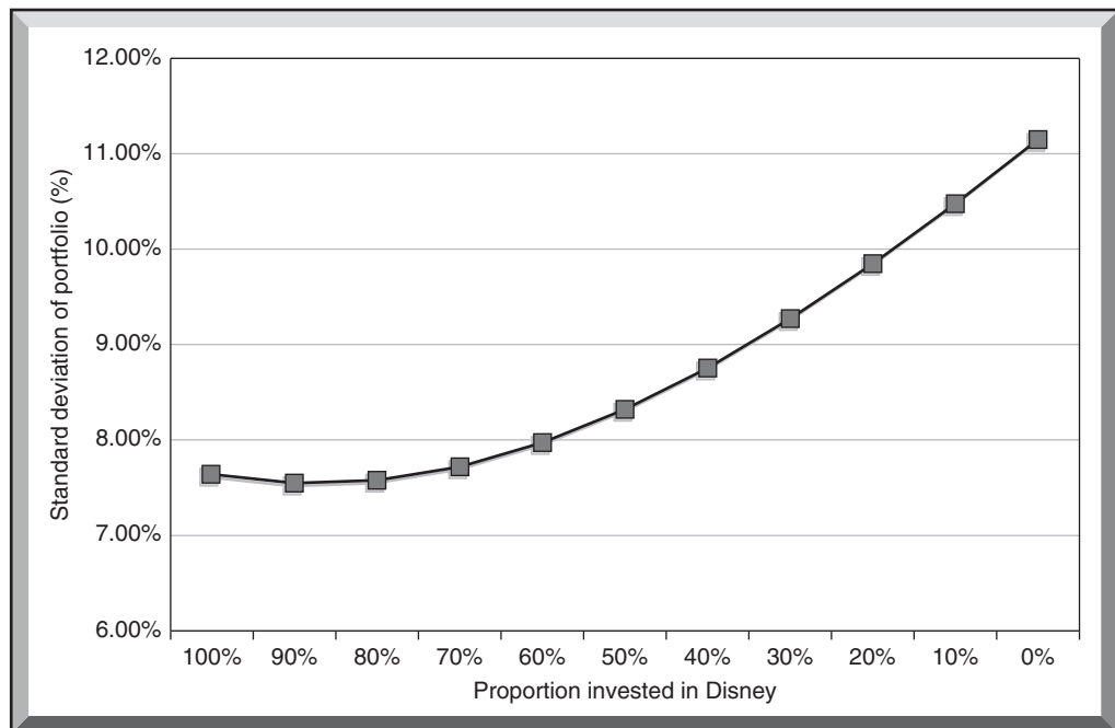
Figure 3.6 Standard Deviation of portfolio of Disney and Vale
