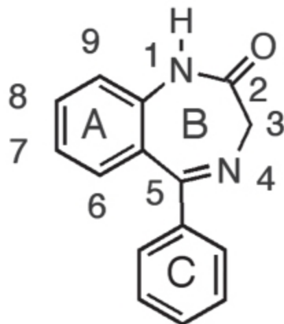
5-Phenyl-1,4-benzodiazepin-2-one backbone
