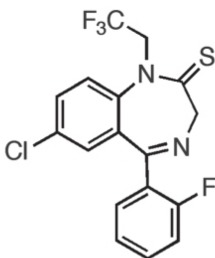
Quazepam
