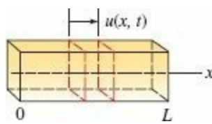
FIGURE 13.4.7 Elastic bar in Problem 11
