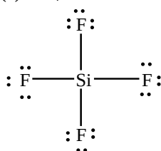
(c) \text{COF}_2
