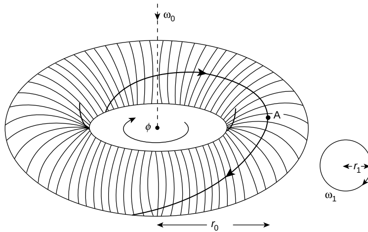
Figure 14.25 Torus in (\dot{x}, t) phase space generated by a system subject to the influence of two perpendicular circular simple harmonic motions. The trajectory of the system spirals on the torus surface
