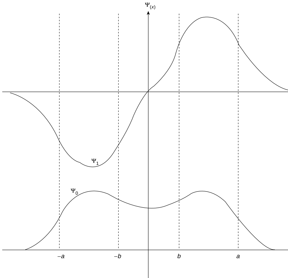
Figure 13.20 When an electron can tunnel between two potential wells (a, b) and -(a, b) it cannot exist in a single energy state. The higher of the two resulting energy states has a greater curvature
