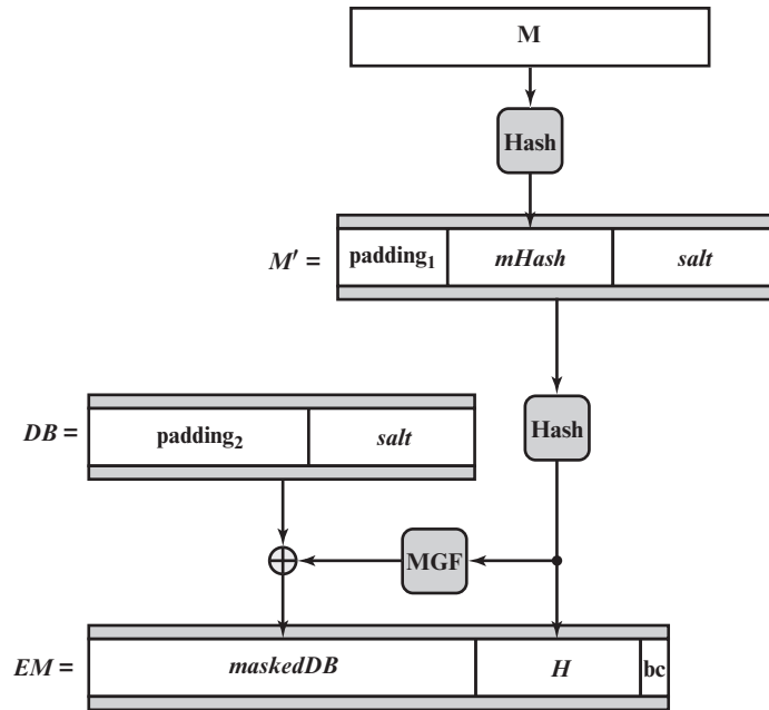
Figure 13.6 RSA-PSS Encoding
