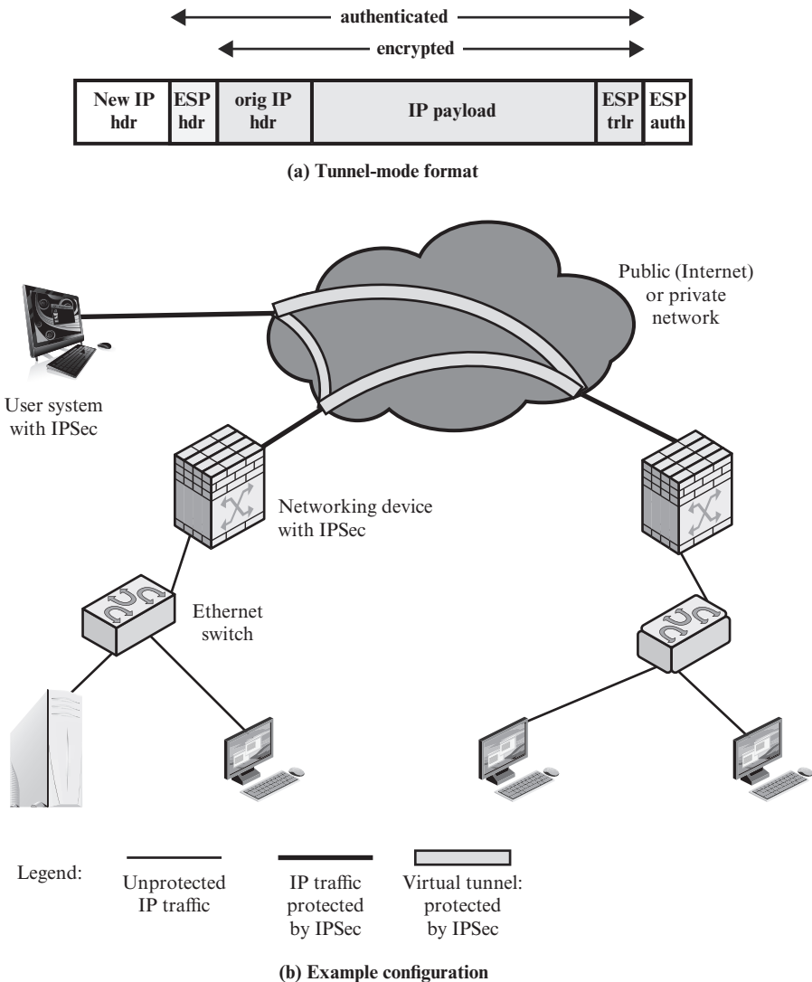
Figure 20.1 An IPSec VPN Scenario
