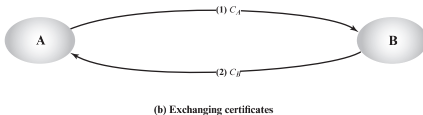
Figure 14.13 Exchange of Public-Key Certificates
