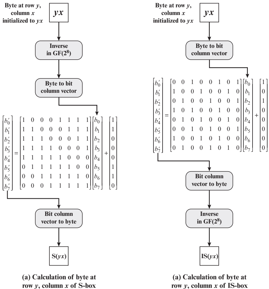
Figure 6.6 Constuction of S-Box and IS-Box
