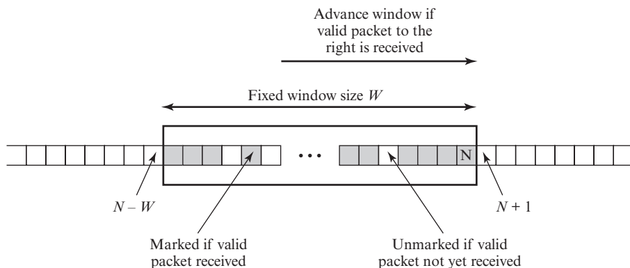
Figure 20.6 Anti-replay Mechanism
