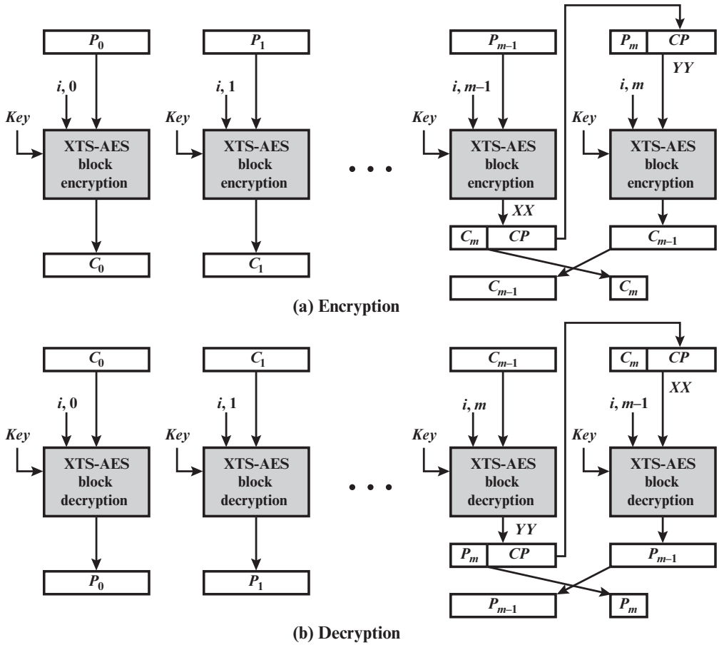
Figure 7.11 XTS-AES Mode
