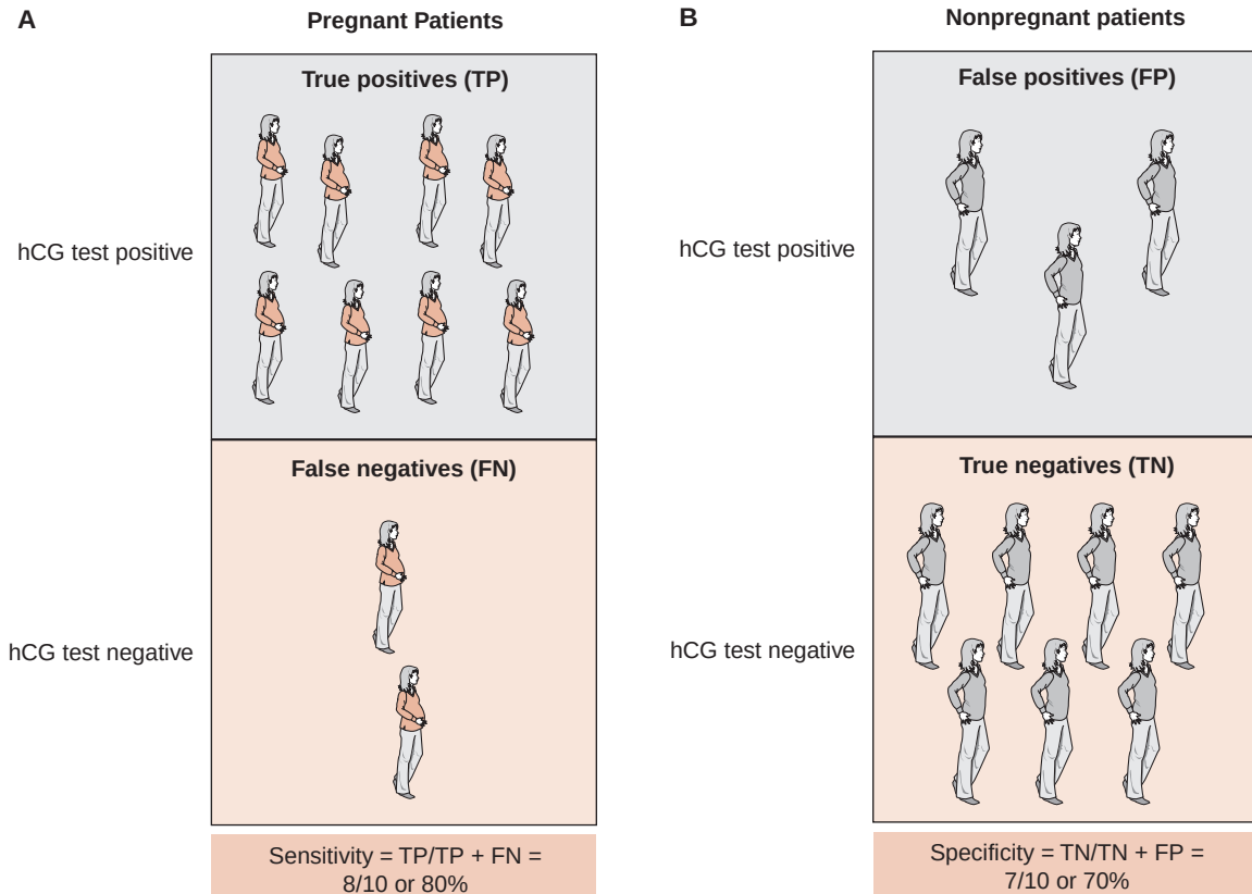
FIGURE 3-24 The sensitivity and specificity of beta-human chorionic gonadotropin ( \beta hCG) for pregnancy. (A) Sensitivity refers to the ability to detect pregnancy. (B) Specificity refers to the ability of the test to correctly classify nonpregnant women. FN, false negative; FP, false positive; TN, true negative; TP, true positive.
