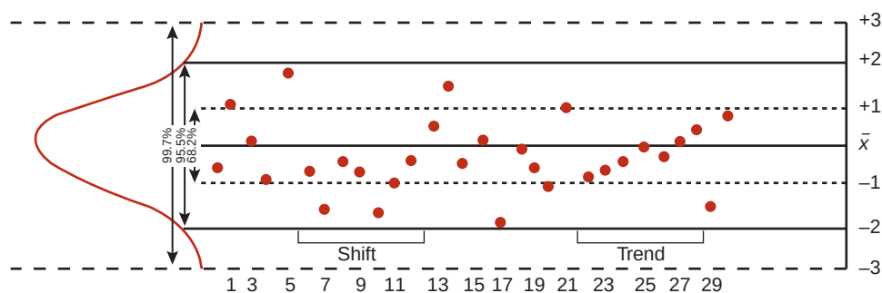
FIGURE 3-18 Control chart showing the relationship of control limits to the Gaussian distribution. Daily values are graphed, and they show examples of a shift, an abrupt change in the analytic process, and a trend, a gradual change in the analytic process.
