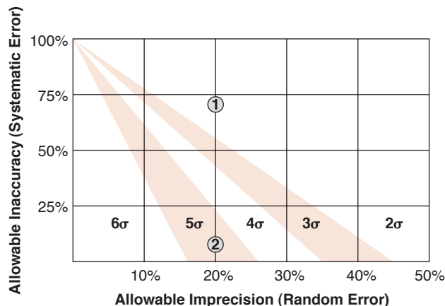
FIGURE 4-7 OPSpecs chart used to determine process performance. The allowable imprecision is plotted against the allowable inaccuracy as percentage of the total allowable error. Assay performance changing from point 1 to point 2 by reducing inaccuracy improves the performance from a 2σ process to a 5σ process.
