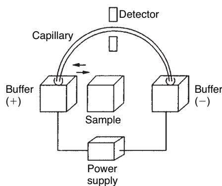
FIGURE 5-24 Schematic of capillary electrophoresis instrumentation. Sample is loaded on the capillary by replacing the anode buffer reservoir with the sample reservoir. (Adapted from Heiger DN. High-Performance Capillary Electrophoresis . Waldbronn, Germany: Hewlett-Packard; 1992.)
