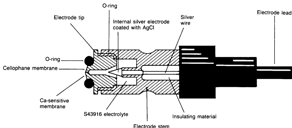
FIGURE 16-6 Diagram of ionized calcium electrode for the ionized calcium analyzer. (Courtesy of Radiometer America, Westlake, OH.)
