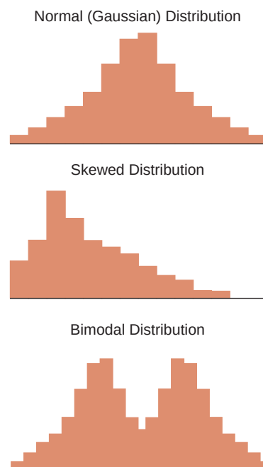
FIGURE 3-6 Examples of normal (Gaussian), skewed, and bimodal distributions. The type of statistical analysis that is performed to analyze the data depends on the distribution (shape).
