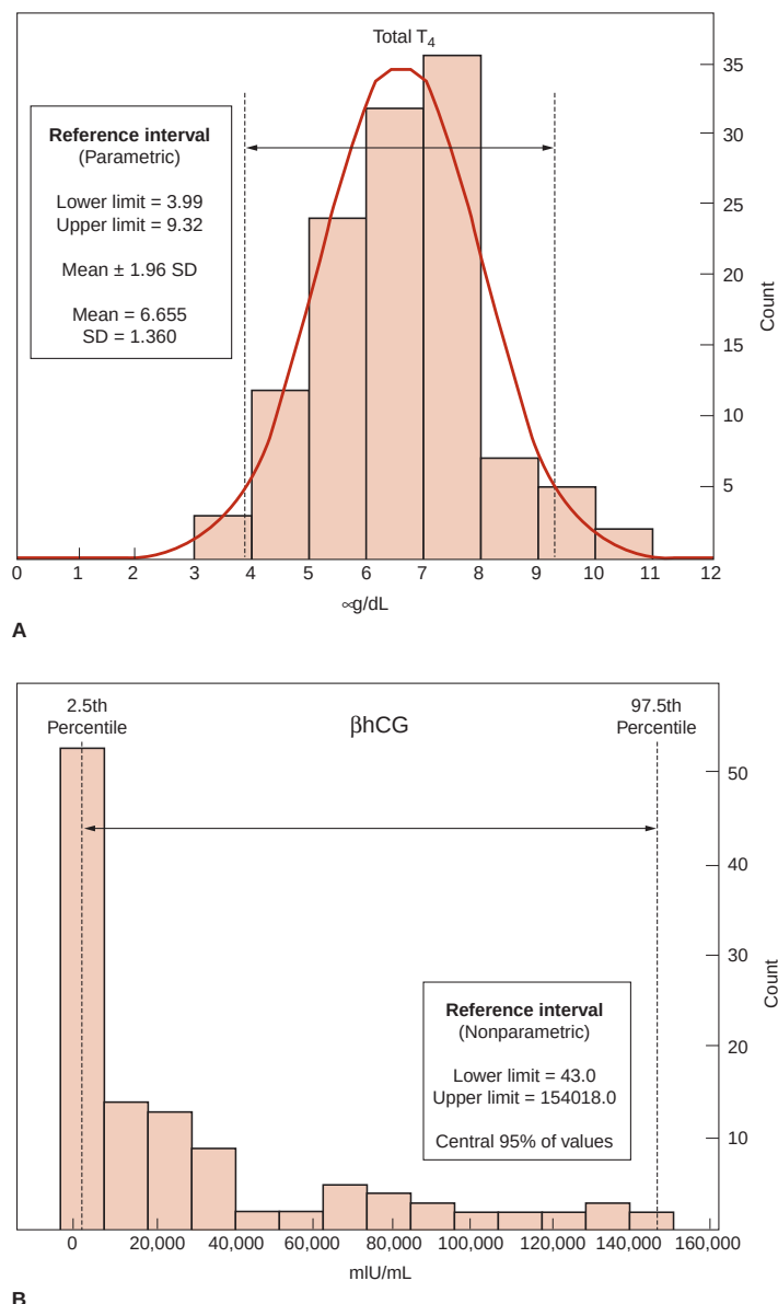
FIGURE 3-20 (A) Histogram of total thyroxine ( \text{TT}_4 ) levels in a real population illustrating a shape indicative of a Gaussian distribution, which is analyzed by parametric statistics. The reference interval is determined from the mean \pm 1.96 SDs. (B) Histogram of beta-human chorionic gonadotropin ( \beta\text{hCG} ) levels in a population of pregnant women demonstrating non-Gaussian data and nonparametric determination of the reference interval. The reference interval is determined from percentiles to include the central 95% of values. Although the selection of a wide range of gestational ages makes this a poor population for a reference interval study, it does demonstrate the application of nonparametric intervals.
