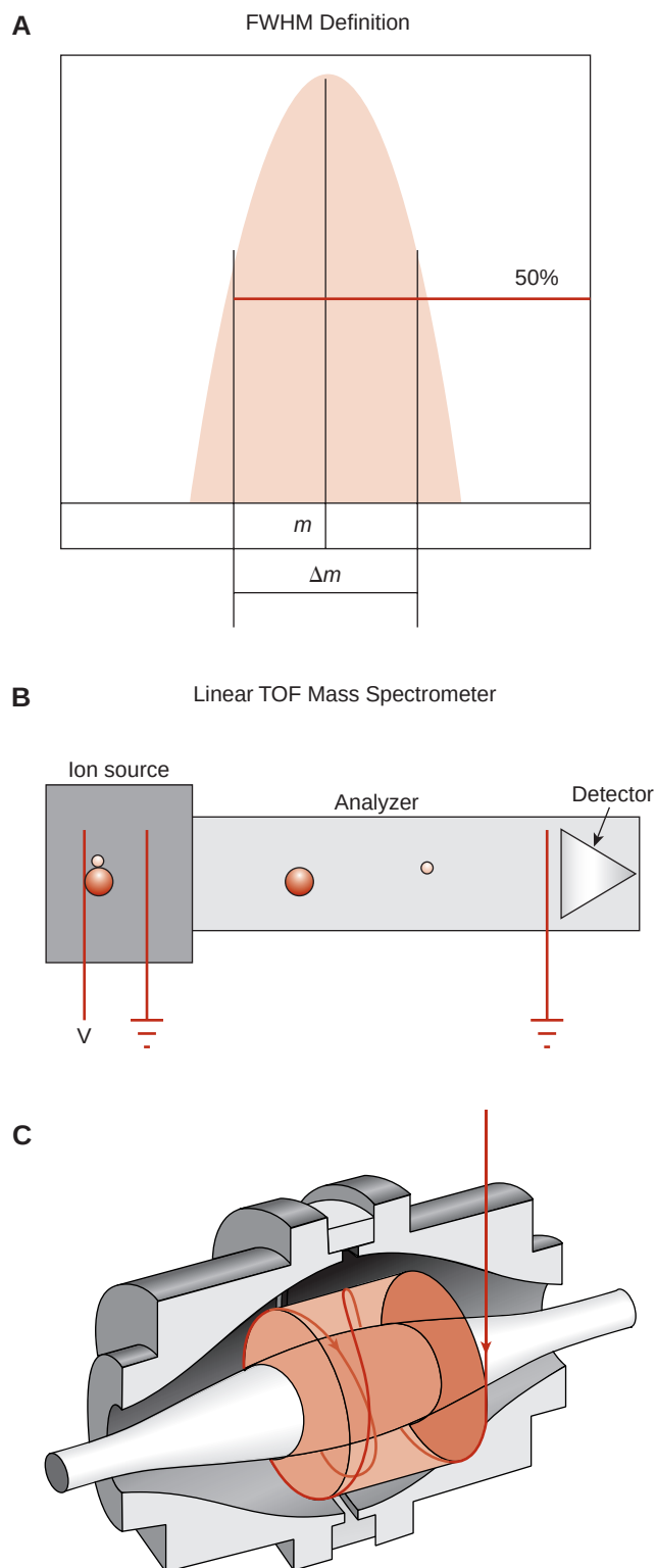
FIGURE 6-16 (A) Pictorial representation of the full width at half maximum (FWHM) definition of mass resolution. Reprinted with permission from Thermo Fisher Scientific. (B) Diagram of the principle of time-of-flight (TOF) mass spectrometers. Reprinted with permission. ( http://msr.dom.wustl.edu/Research/MALDI_TOF_Mass_Spec_and_Proteomics/Time-of-Flight_Mass_Spectrometry_Fundamentals.htm ) (C) Diagram of Orbitrap mass spectrometry. Reprinted with permission from Thermo Fisher Scientific.
