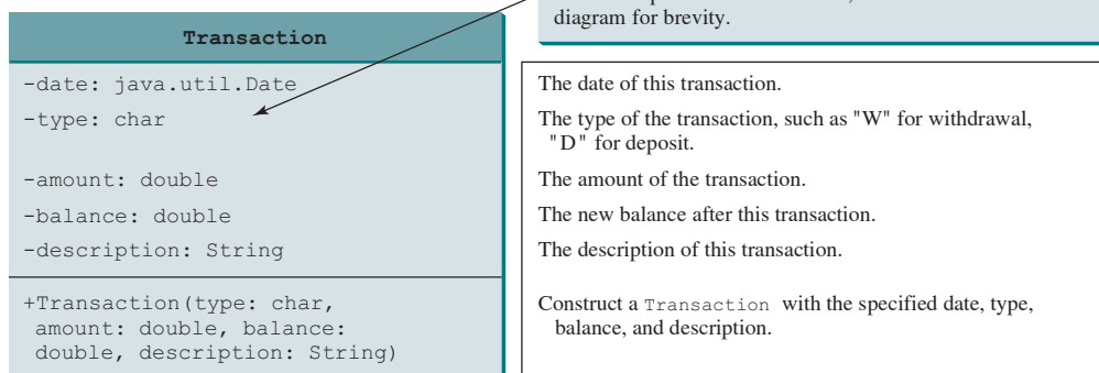
FIGURE 11.6 The Transaction class describes a transaction for a bank account.
