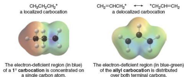
Figure 16.2 Electrostatic potential maps for a localized and a delocalized carbocation
