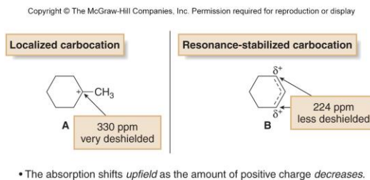
Figure 16.3 ^{13}\text{C} chemical shifts for a localized and a resonance-stabilized carbocation
